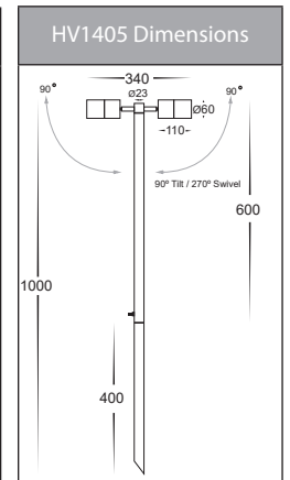
HV1405T-SS316
