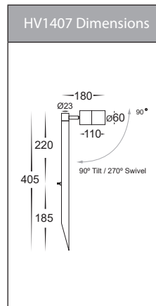
HV1407T-SS316
