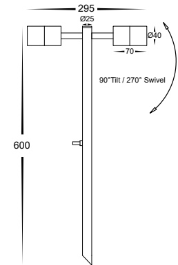
HV1425 Dimensions
