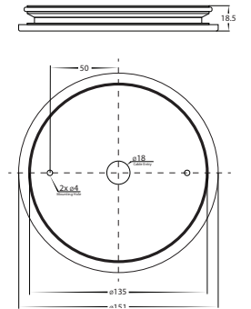
Mounting Base for HV2929
