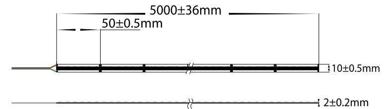
IP54 10mm (W) x 3mm (H) LED Strip Dimensions
