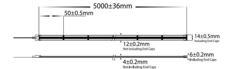
IP67 14mm (W) x 6mm (H) LED Strip Dimensions
