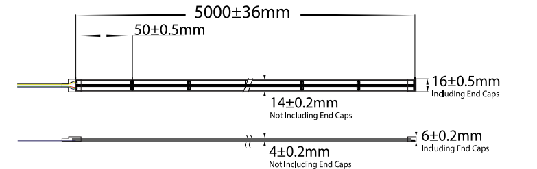
IP67 16mm (W) x 6mm (H) LED Strip Dimensions
