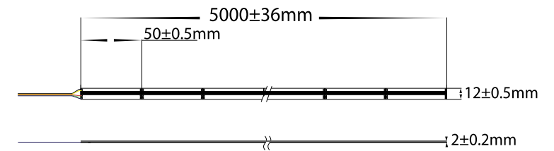
IP54 12mm (W) x 3mm (H) LED Strip Dimensions
