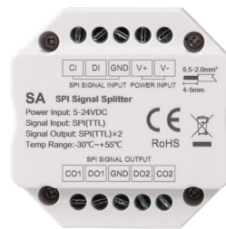
2 Channel HV9104-SPI-2CH
