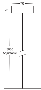
HV5844-PDT Dimensions
