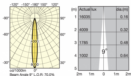
DOT 70/20W/PGJ5/NARROW
