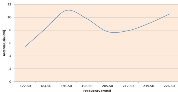
01ACD12 VHF Gain (dBi) vs. Freq (MHz)
