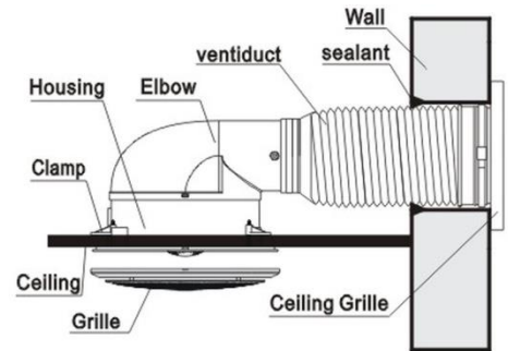
Fig. 2 – Installing duct if required
